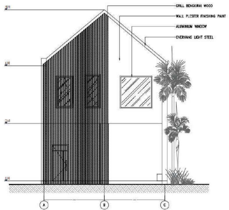
FRONT ELEVATION
