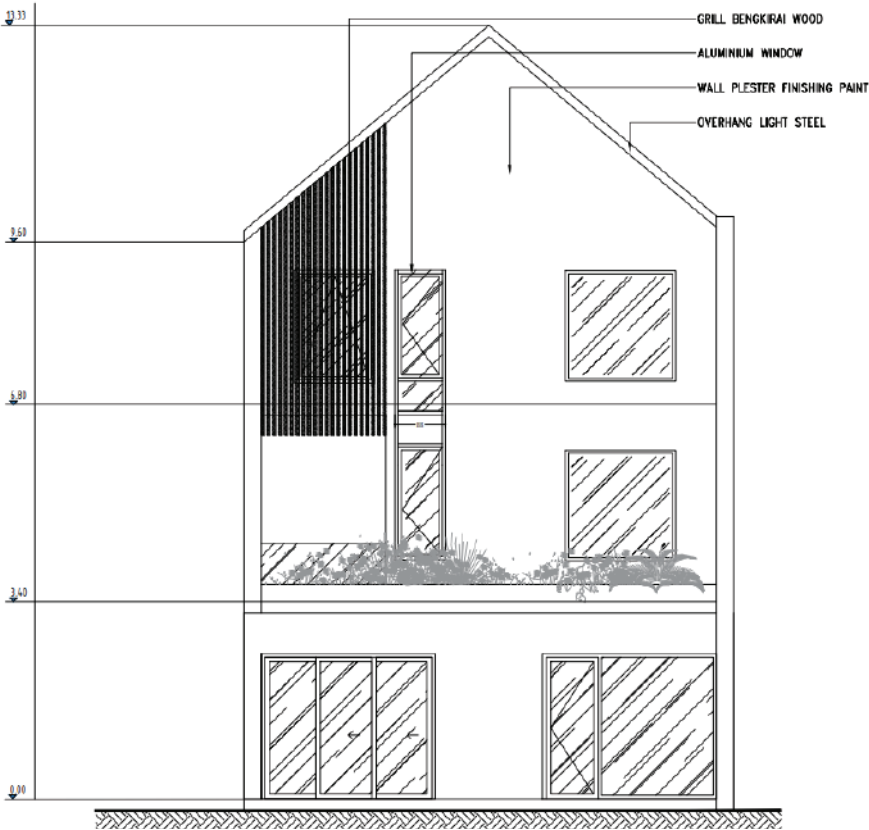
REAR ELEVATION
