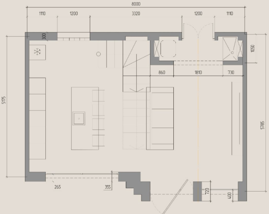
1 st FLOOR
