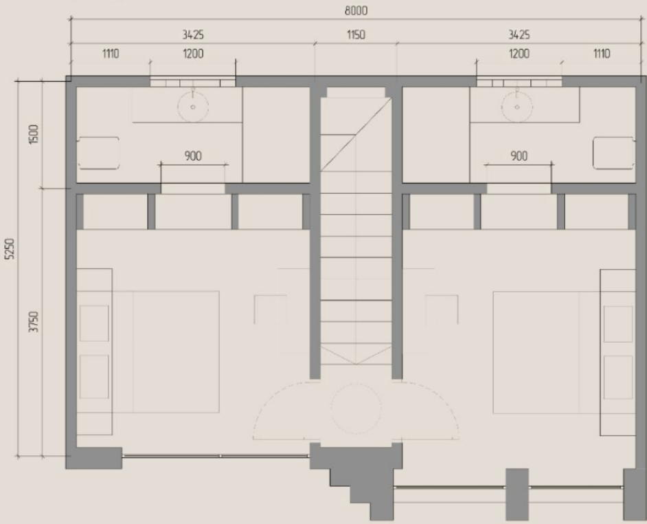
2 nd FLOOR
