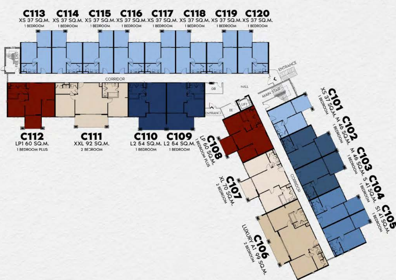
1 ST FLOOR
